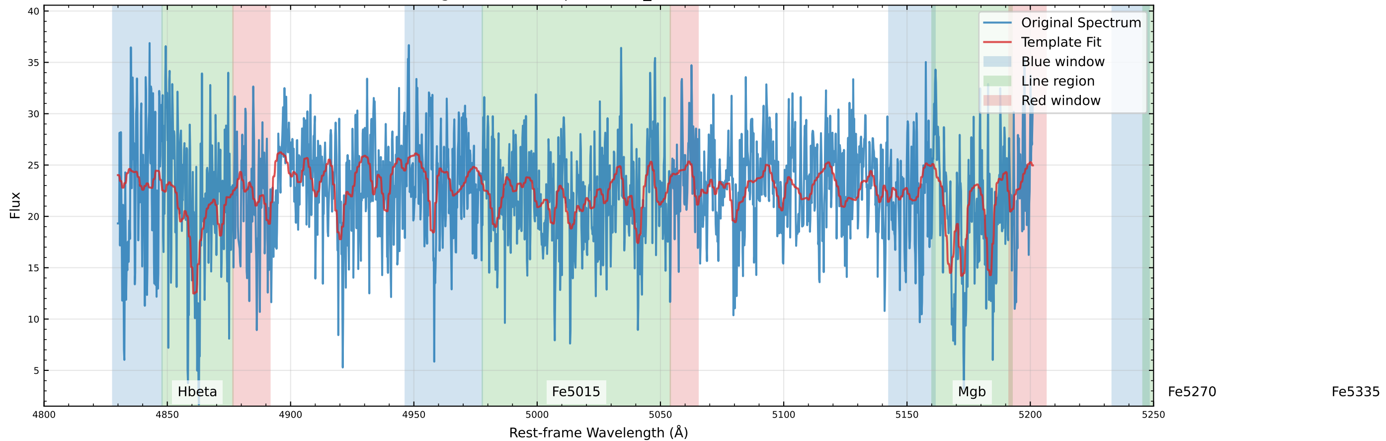
Original Data Comparison (v_star=66.9 km/s)
