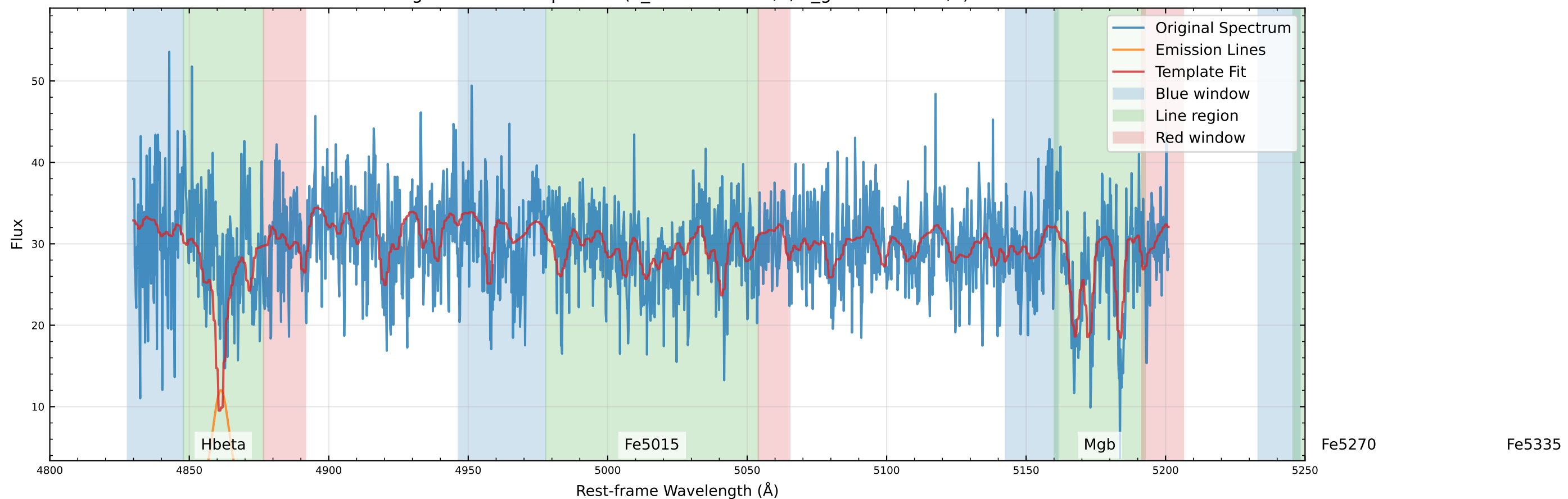
Original Data Comparison (v_star=42.8 km/s, v_gas=-12.6 km/s)
