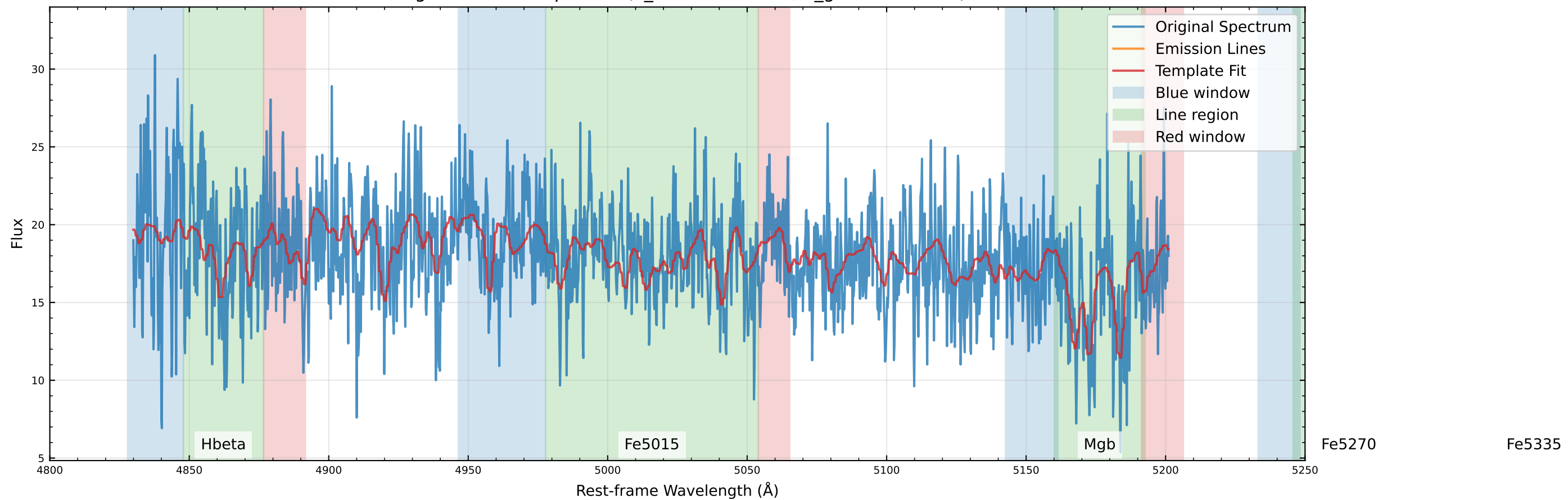
Original Data Comparison (v_star=29.0 km/s, v_gas=36.9 km/s)
