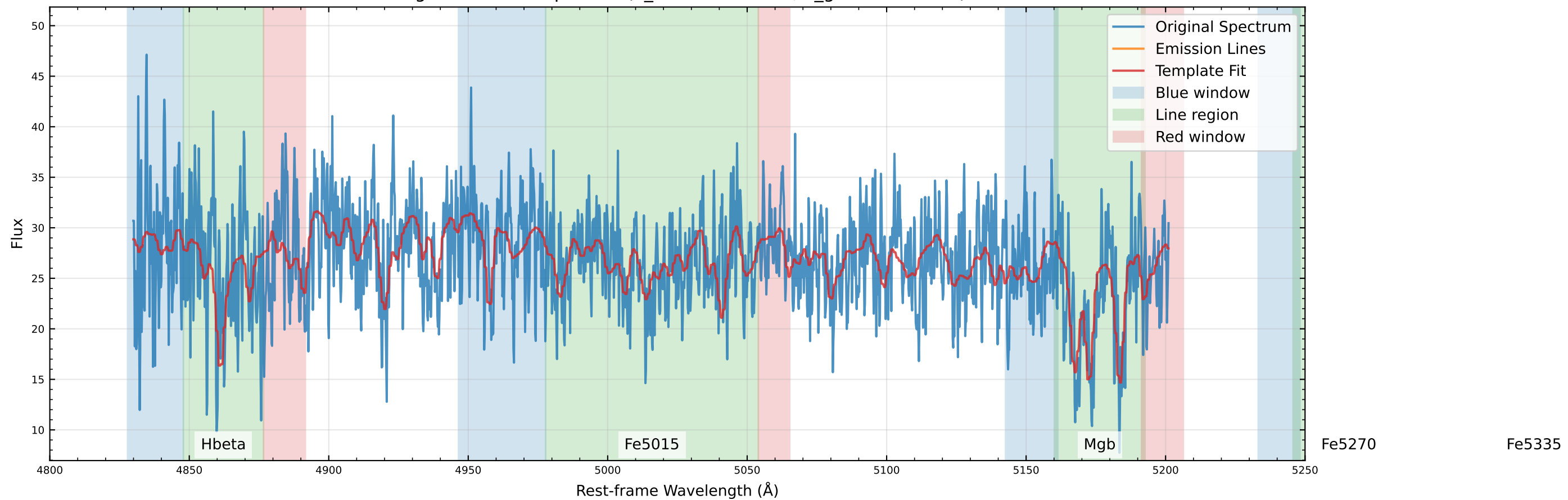
Original Data Comparison (v_star=36.4 km/s, v_gas=42.2 km/s)
