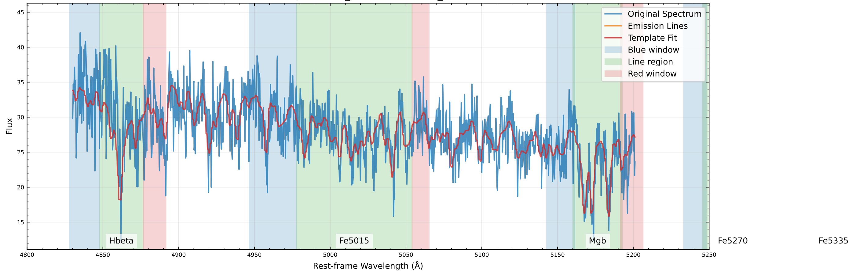
Original Data Comparison (v_star=35.7 km/s, v_gas=-210.2 km/s)
