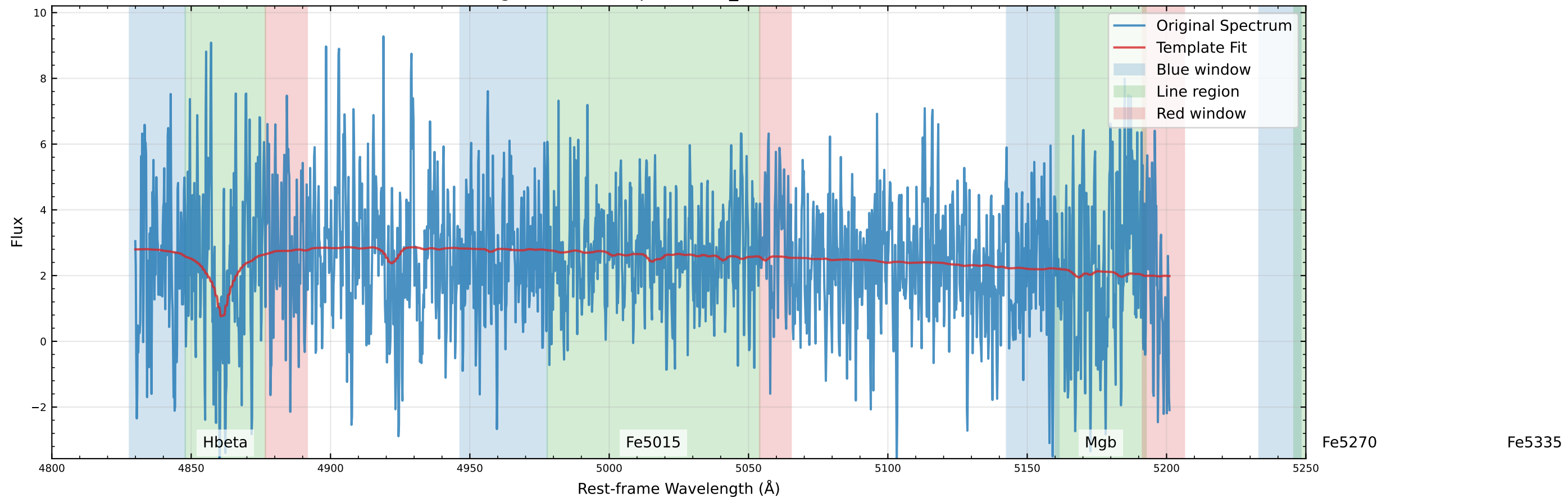
Original Data Comparison (v_star=25.3 km/s)
