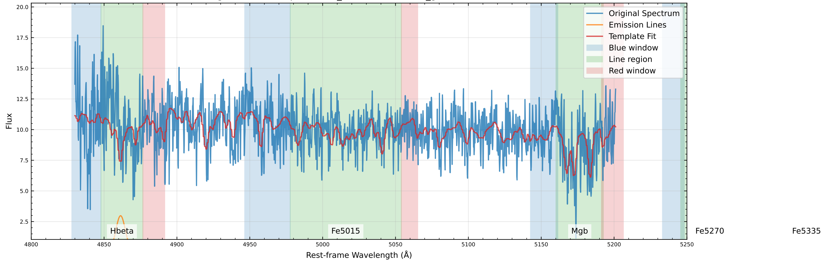
Original Data Comparison (v_star=29.2 km/s, v_gas=-270.8 km/s)
