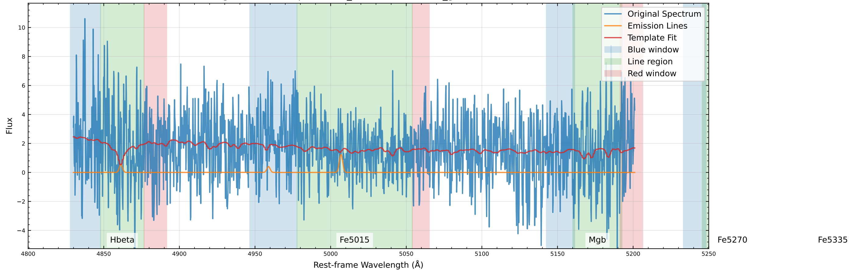
Original Data Comparison (v_star=-33.4 km/s, v_gas=-23.6 km/s)
