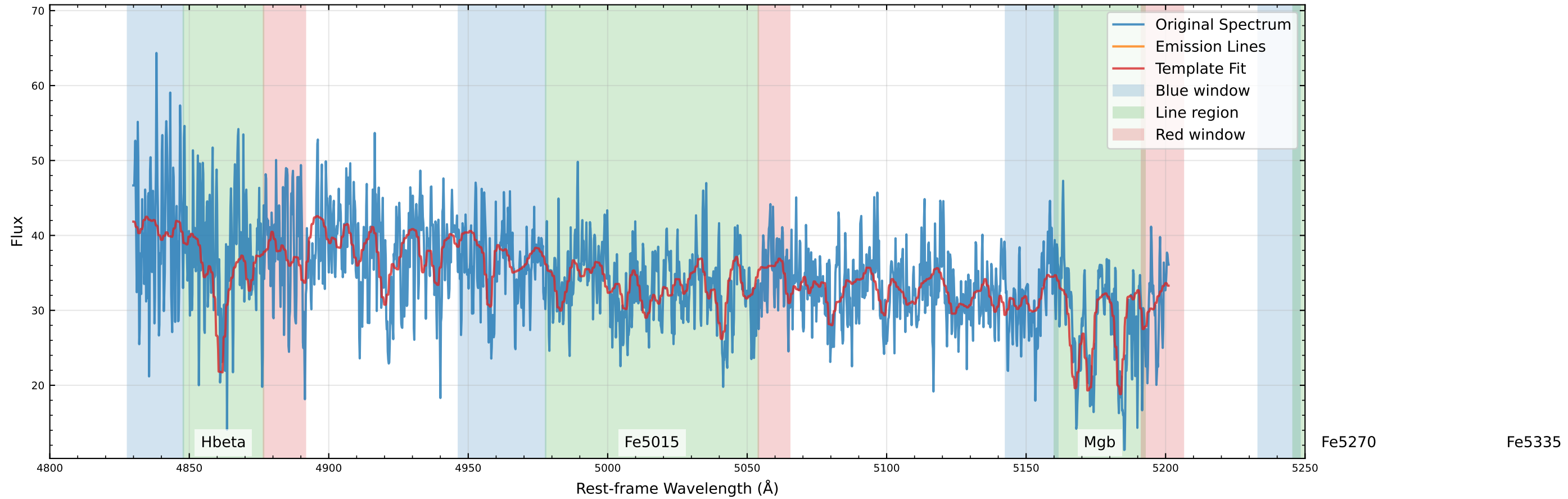
Original Data Comparison ( v_{\text{star}}=57.5 km/s, v_{\text{gas}}=225.2 km/s)
