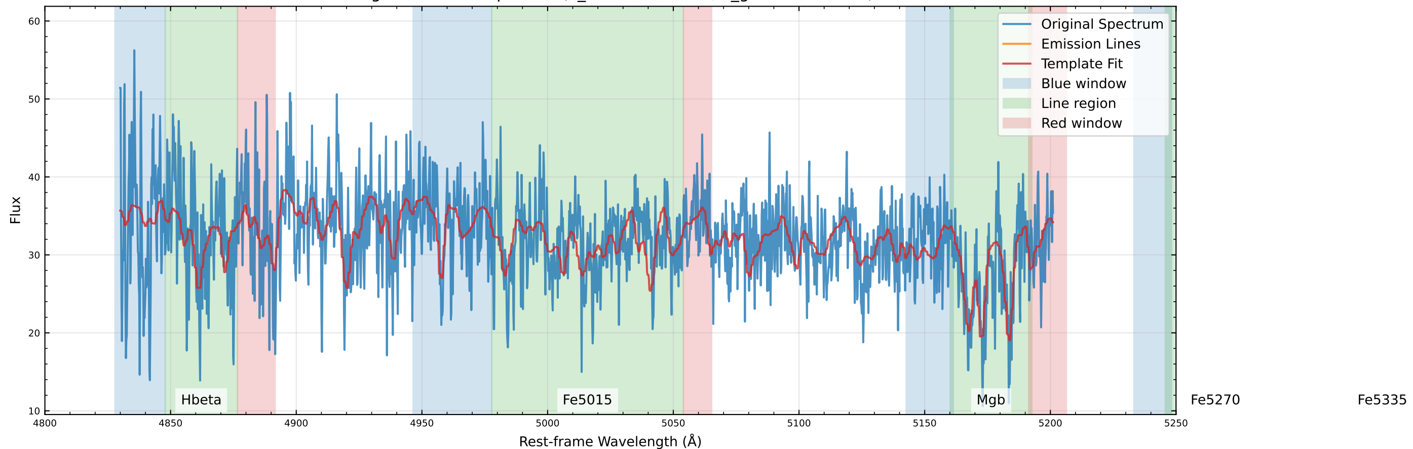
Original Data Comparison (v_star=24.4 km/s, v_gas=-48.8 km/s)
