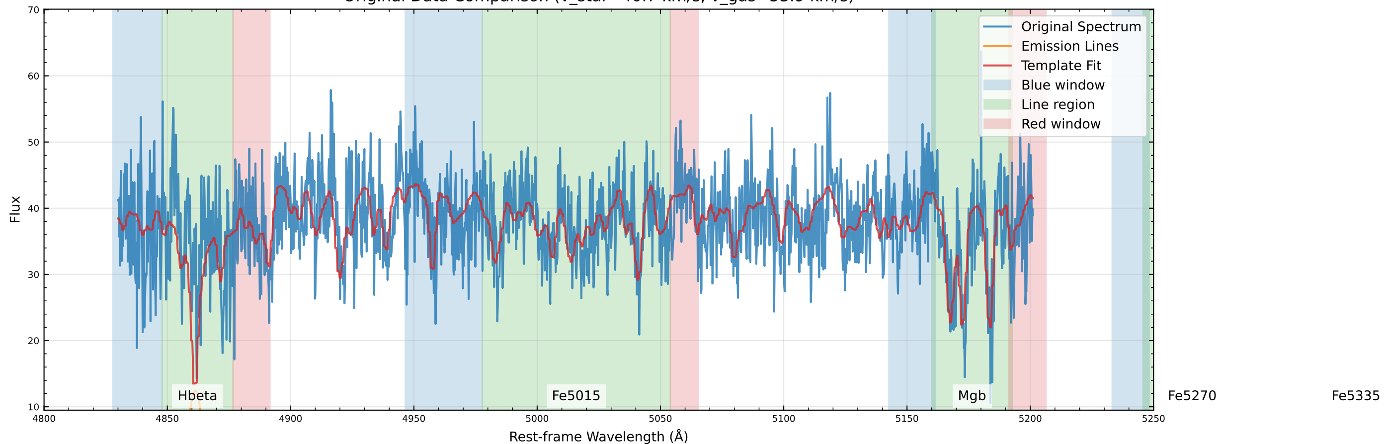
Original Data Comparison (v_star=40.7 km/s, v_gas=53.9 km/s)
