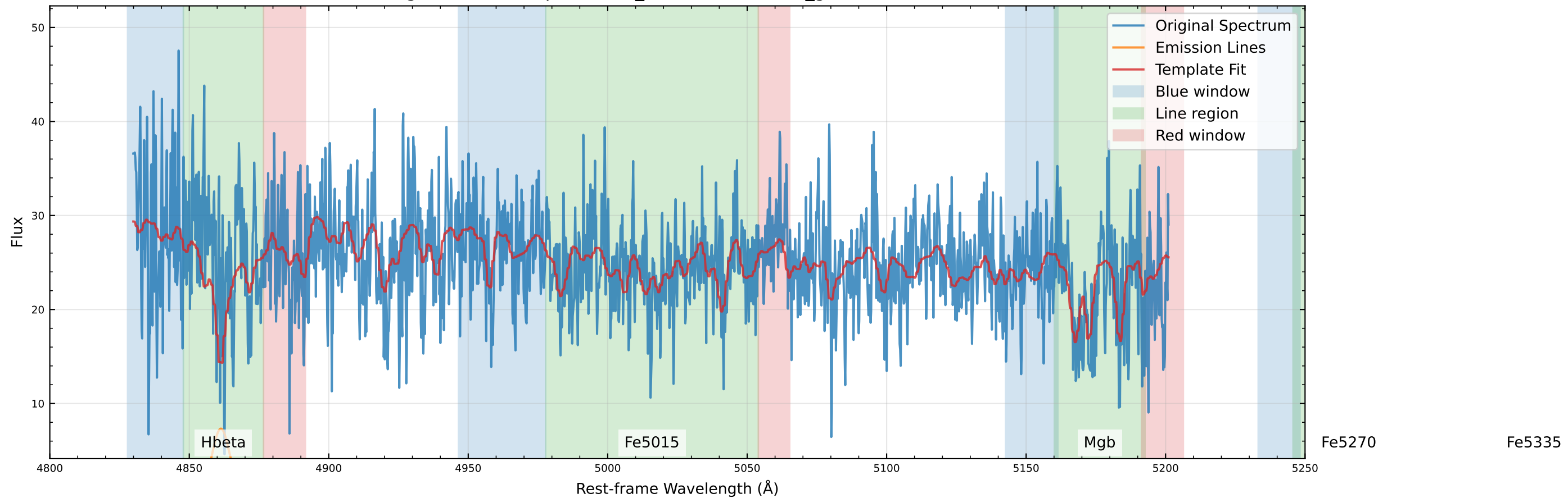
Original Data Comparison (v_star=48.8 km/s, v_gas=-224.2 km/s)
