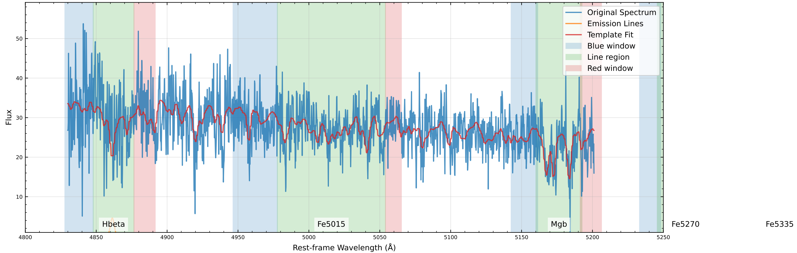
Original Data Comparison (v_star=42.7 km/s, v_gas=-11.5 km/s)
