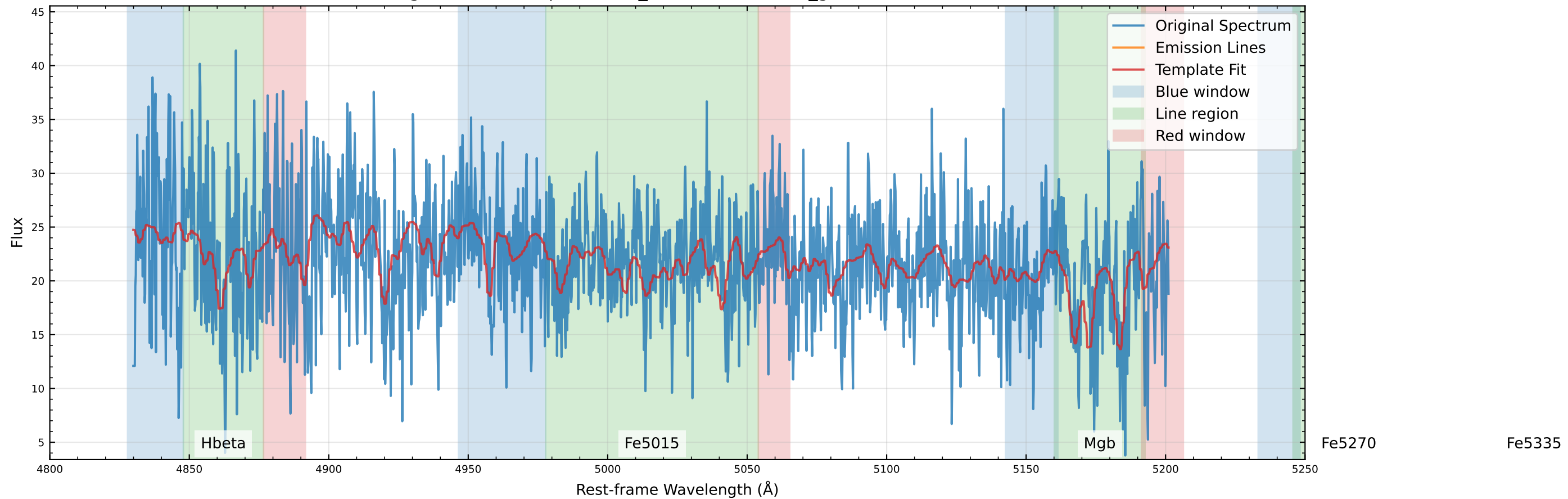
Original Data Comparison ( v_{\text{star}}=65.4 km/s, v_{\text{gas}}=111.7 km/s)
