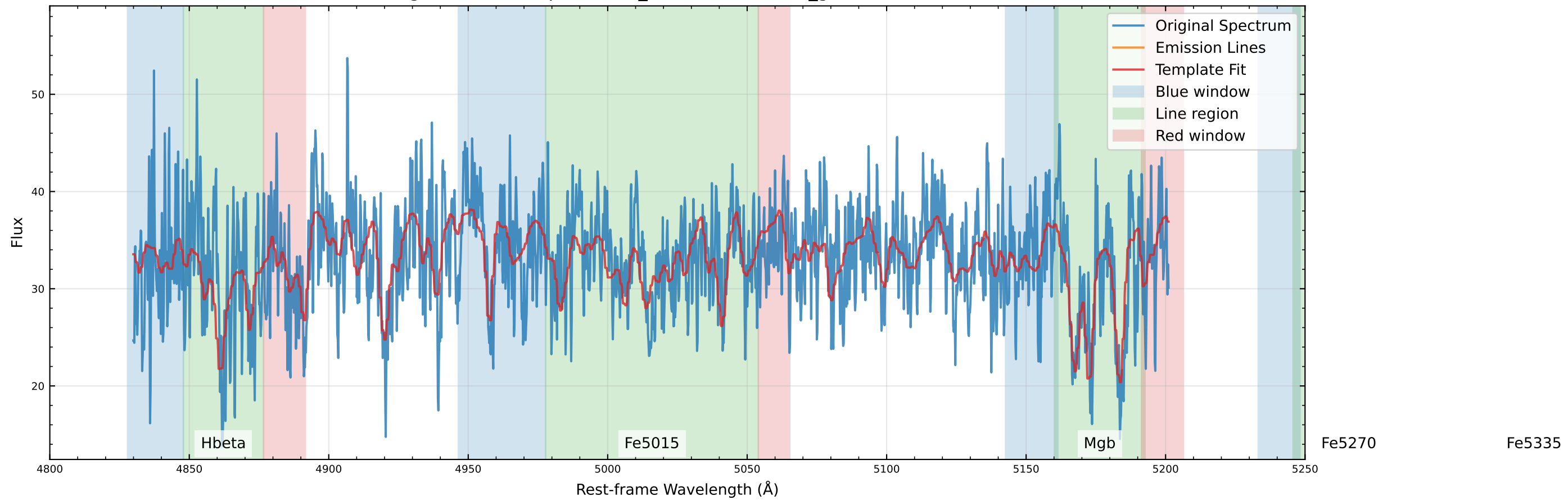
Original Data Comparison ( v_{\text{star}}=29.4 km/s, v_{\text{gas}}=183.1 km/s)
