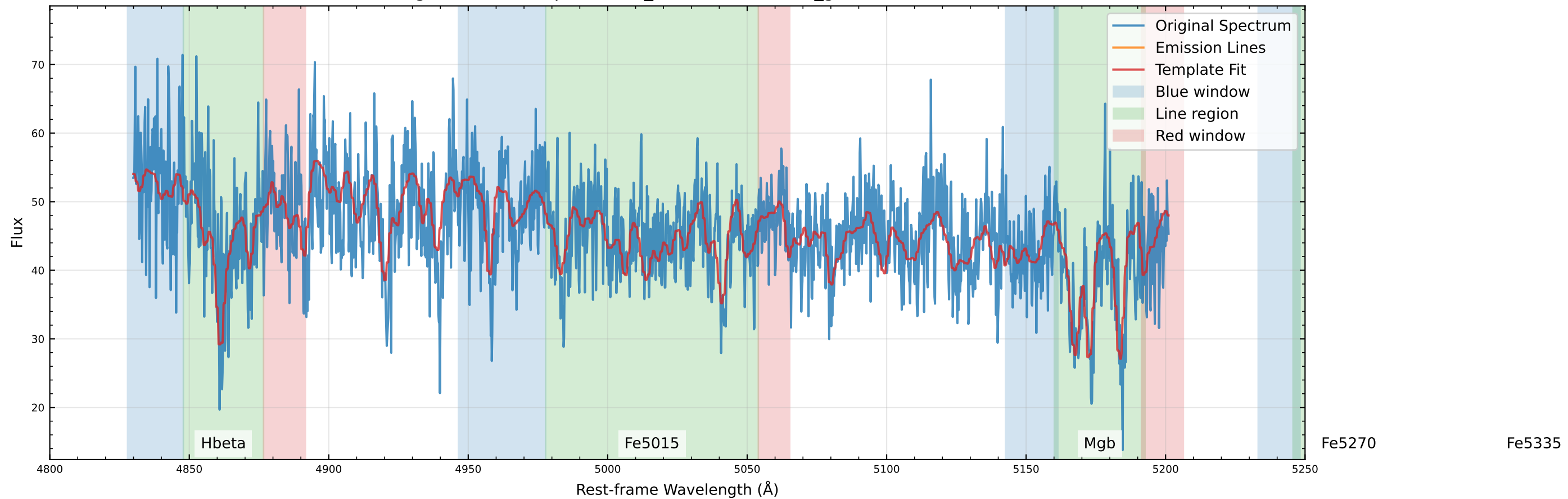
Original Data Comparison (v_star=42.6 km/s, v_gas=42.4 km/s)
