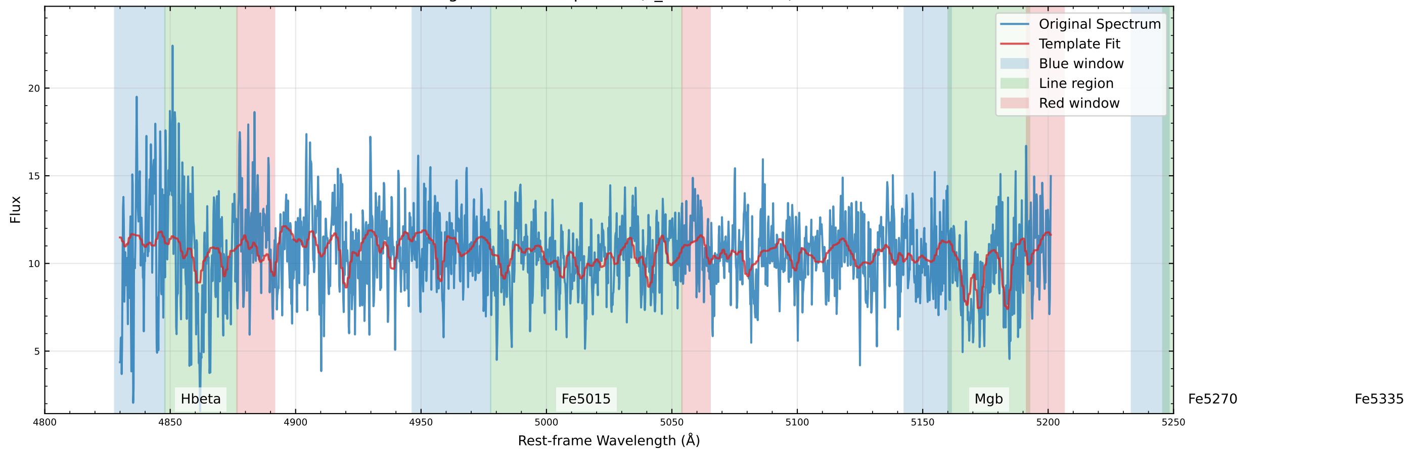
Original Data Comparison (v_star=75.3 km/s)
