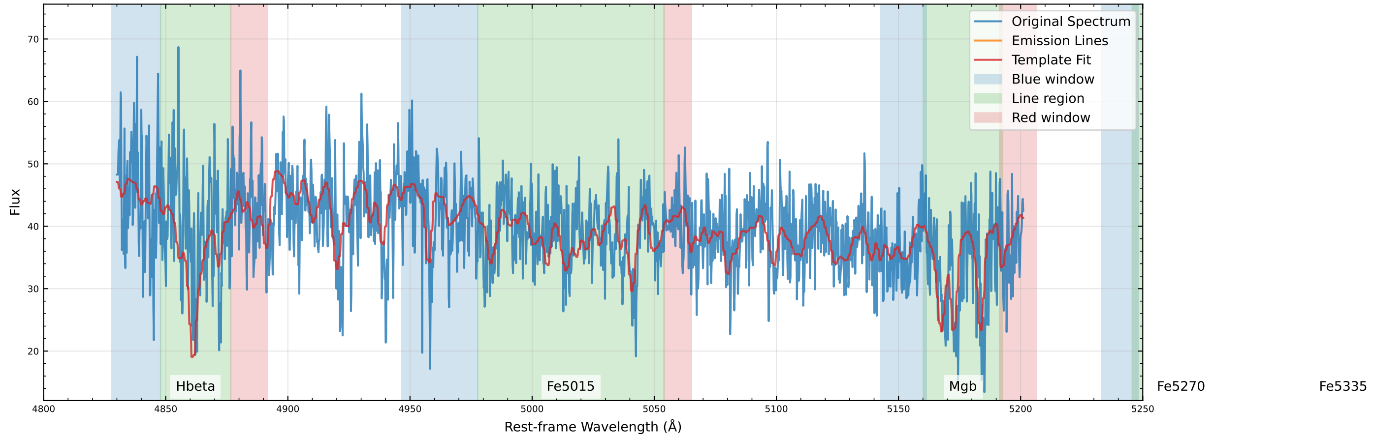
Original Data Comparison (v_star=65.8 km/s, v_gas=49.7 km/s)
