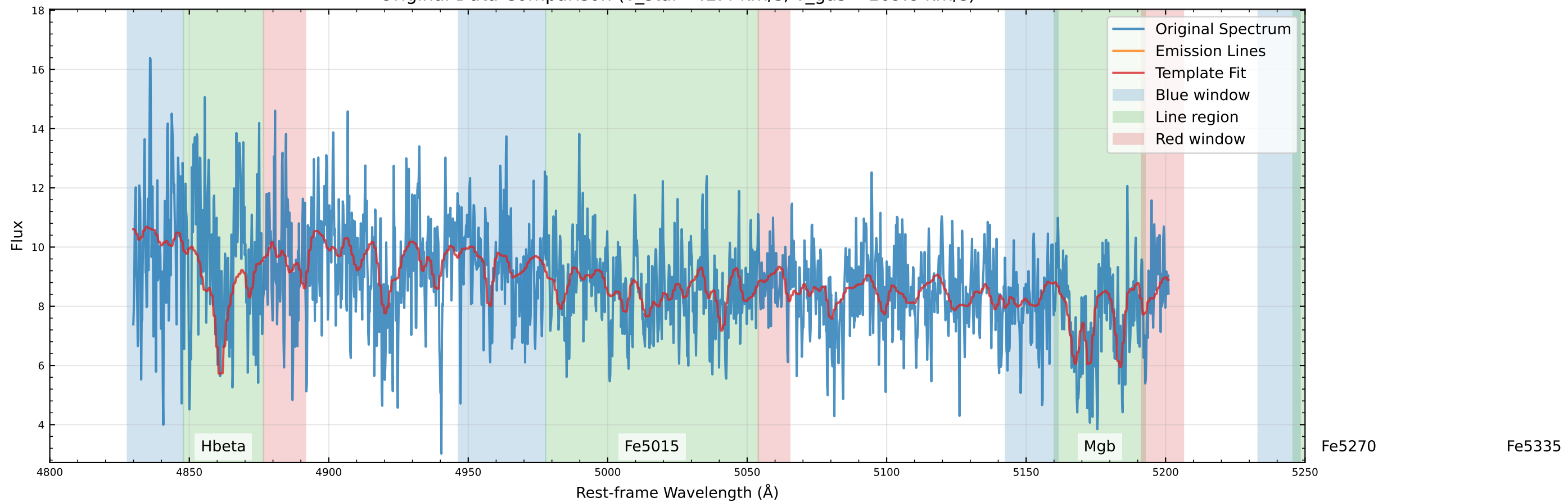
Original Data Comparison (v_star=42.4 km/s, v_gas=-169.8 km/s)
