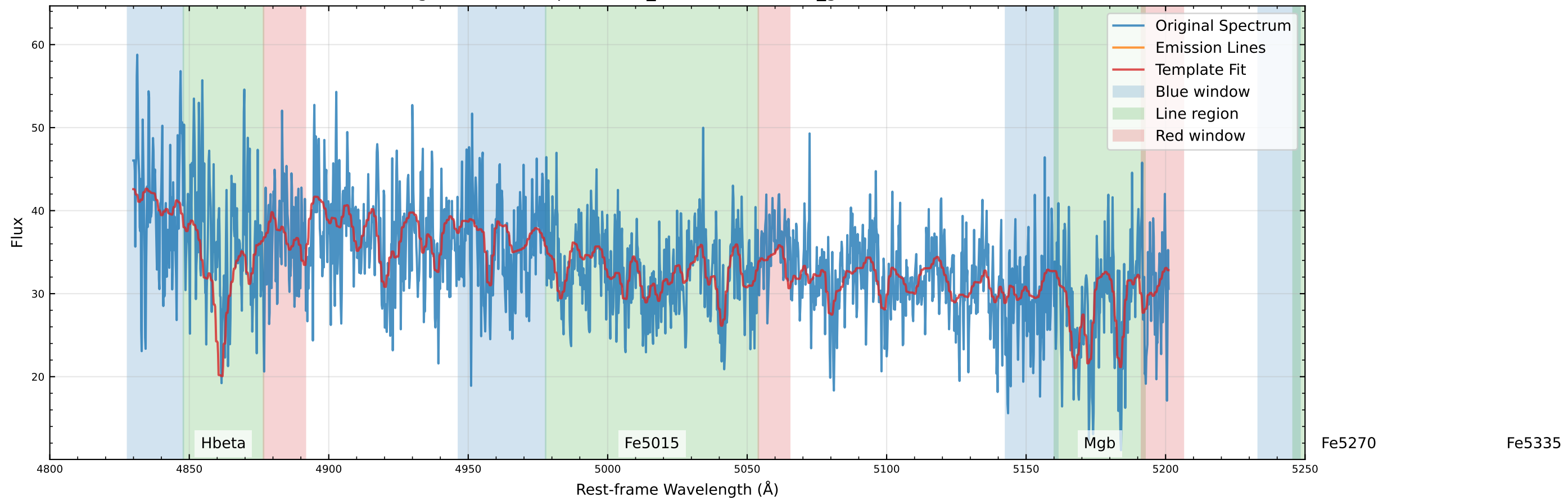
Original Data Comparison (v_star=42.6 km/s, v_gas=-7.0 km/s)
