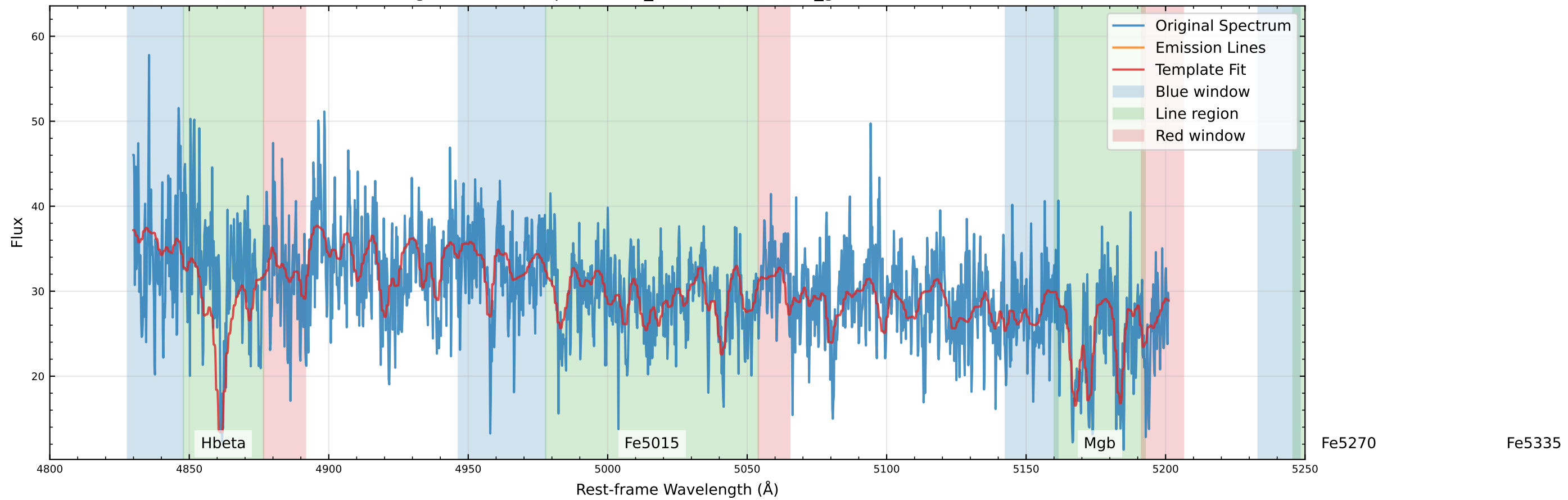
Original Data Comparison (v_star=38.4 km/s, v_gas=48.0 km/s)
