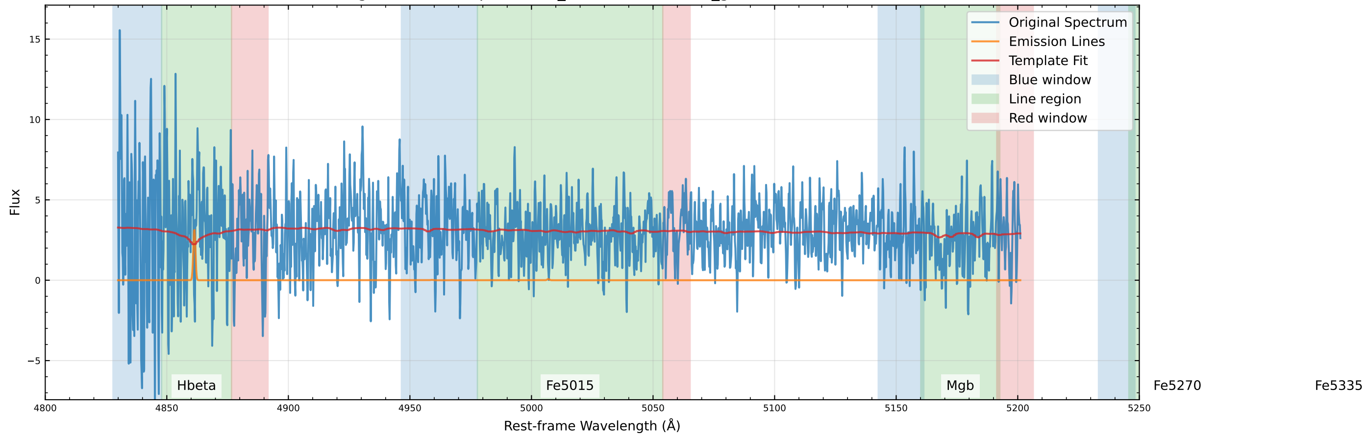
Original Data Comparison (v_star=-74.8 km/s, v_gas=-59.1 km/s)
