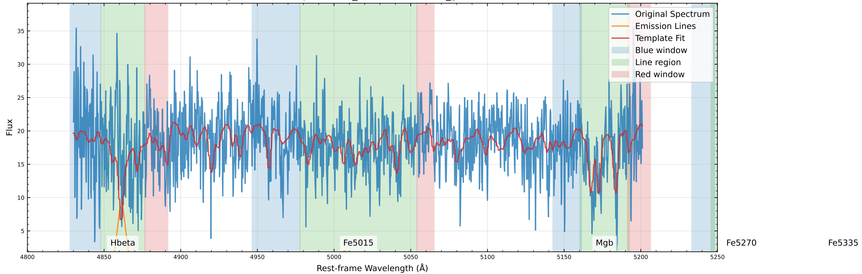
Original Data Comparison (v_star=35.8 km/s, v_gas=-95.6 km/s)
