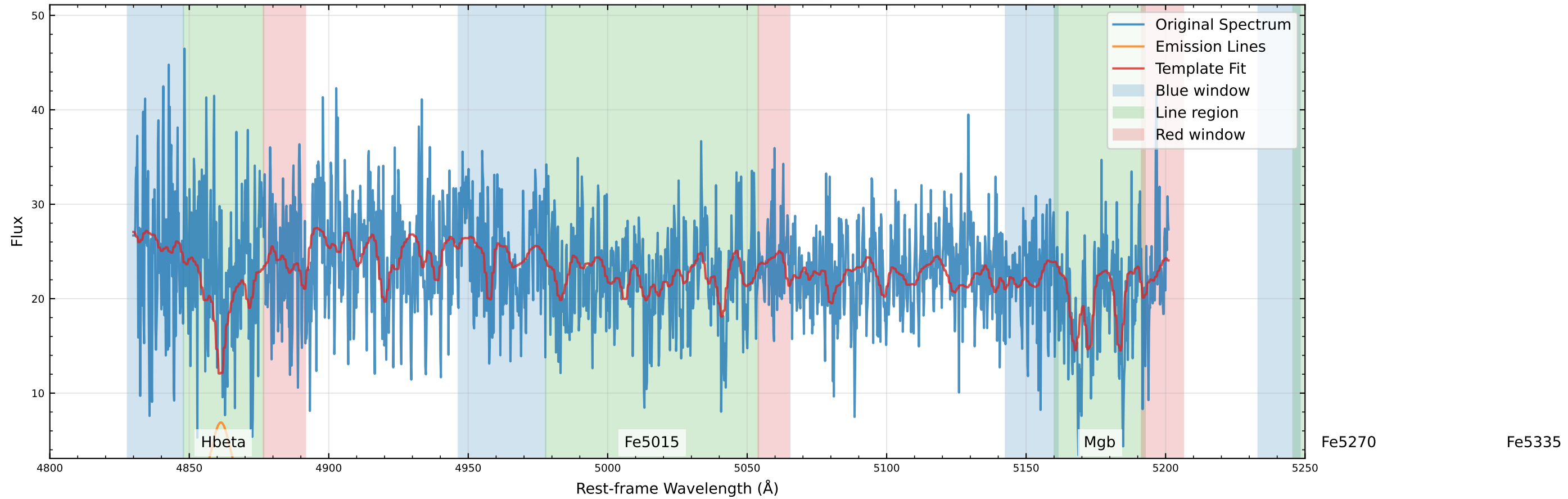
Original Data Comparison (v_star=65.7 km/s, v_gas=-99.1 km/s)
