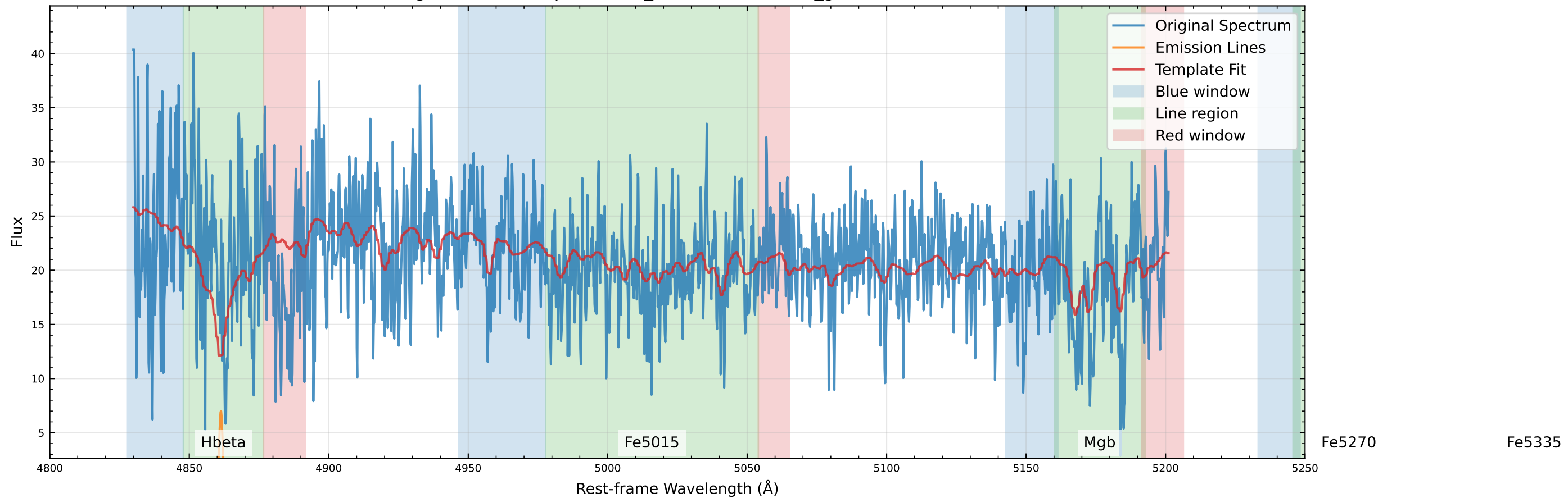
Original Data Comparison (v_star=52.2 km/s, v_gas=12.9 km/s)
