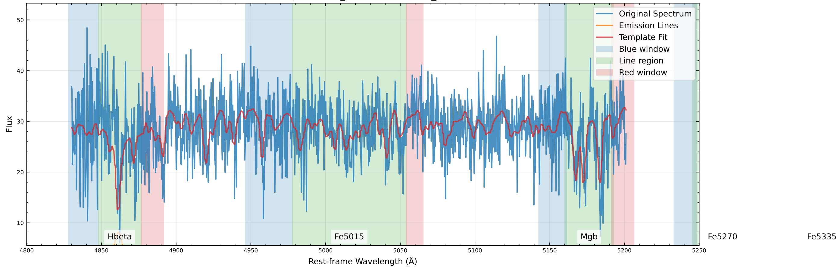
Original Data Comparison (v_star=43.2 km/s, v_gas=-146.2 km/s)
