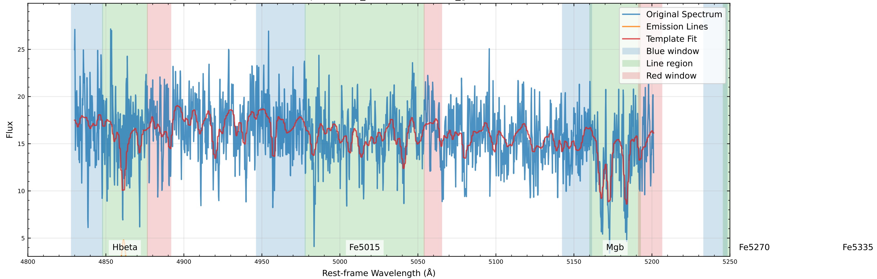
Original Data Comparison (v_star=11.5 km/s, v_gas=75.0 km/s)
