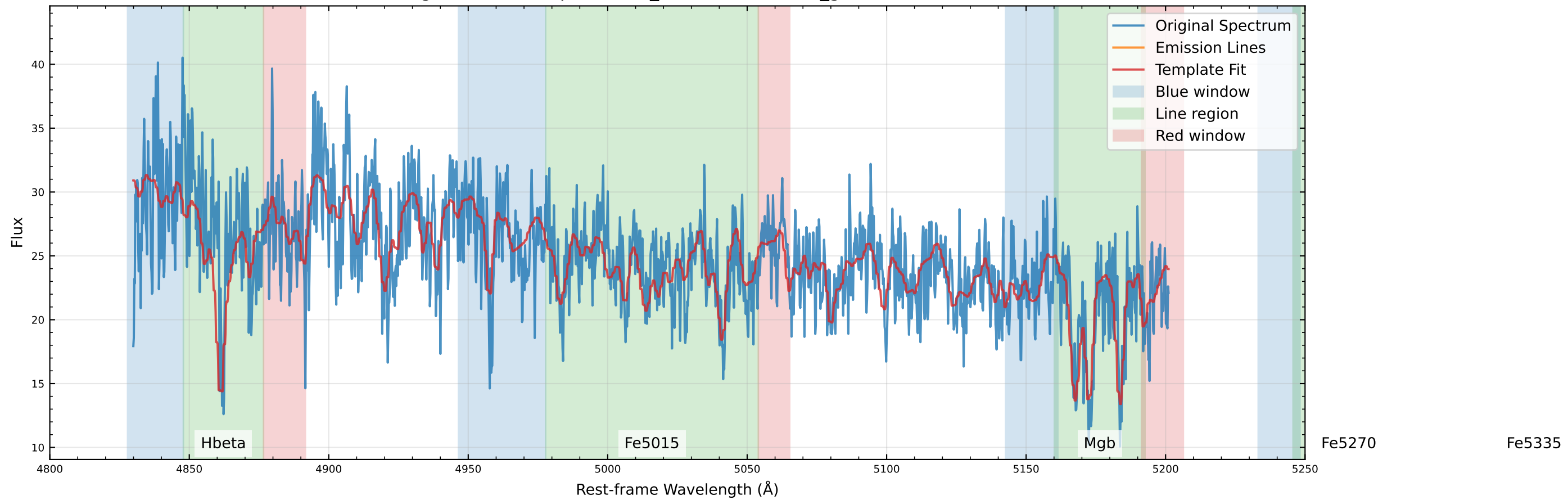
Original Data Comparison (v_star=30.6 km/s, v_gas=1.1 km/s)
