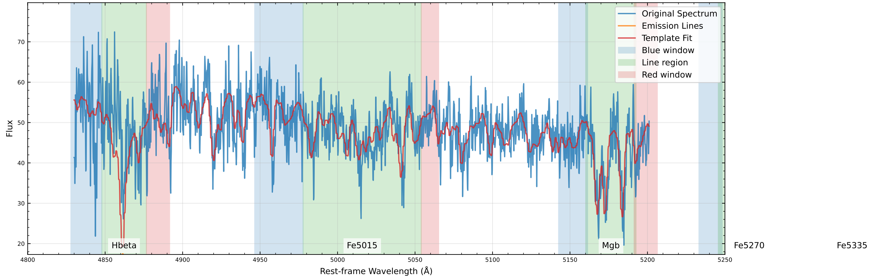
Original Data Comparison (v_star=47.8 km/s, v_gas=-65.6 km/s)
