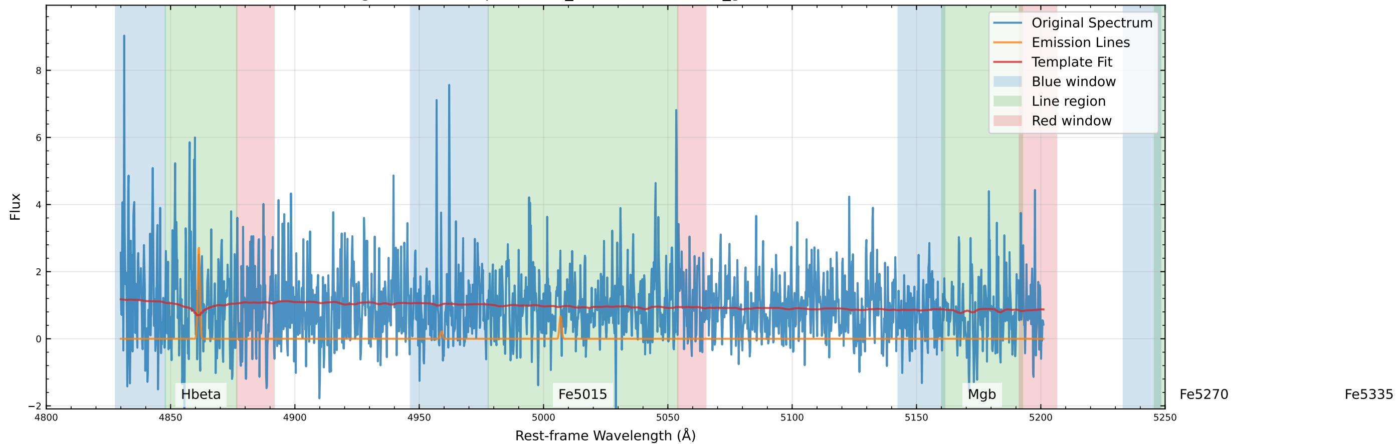
Original Data Comparison (v_star=-52.5 km/s, v_gas=-109.7 km/s)
