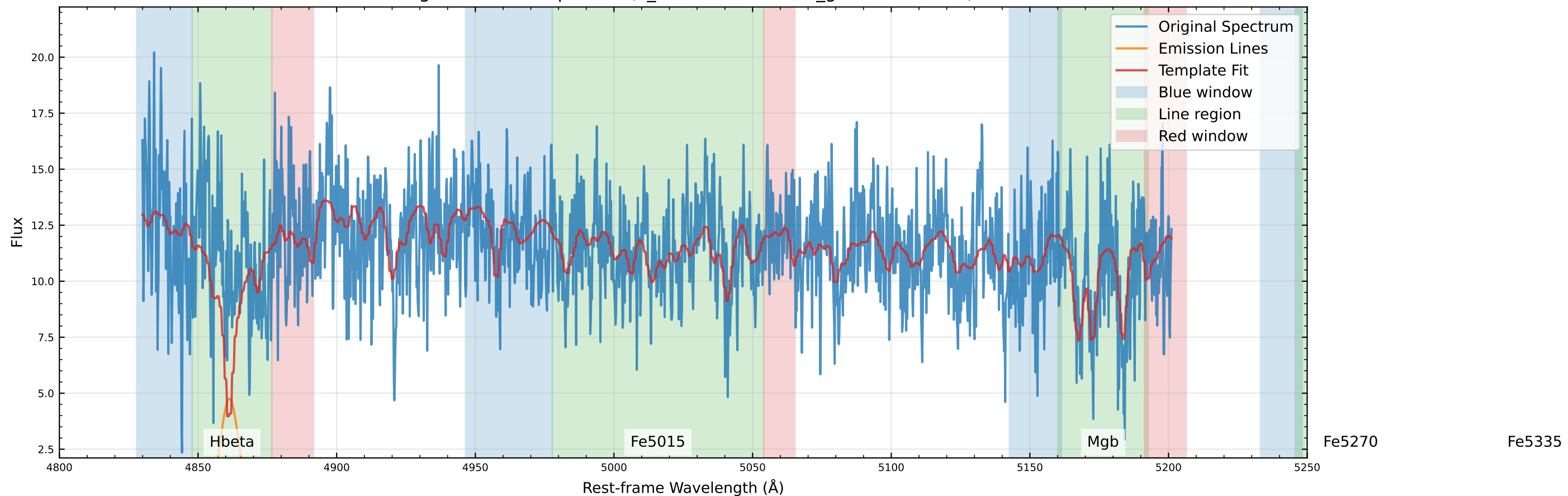
Original Data Comparison (v_star=25.8 km/s, v_gas=-19.8 km/s)
