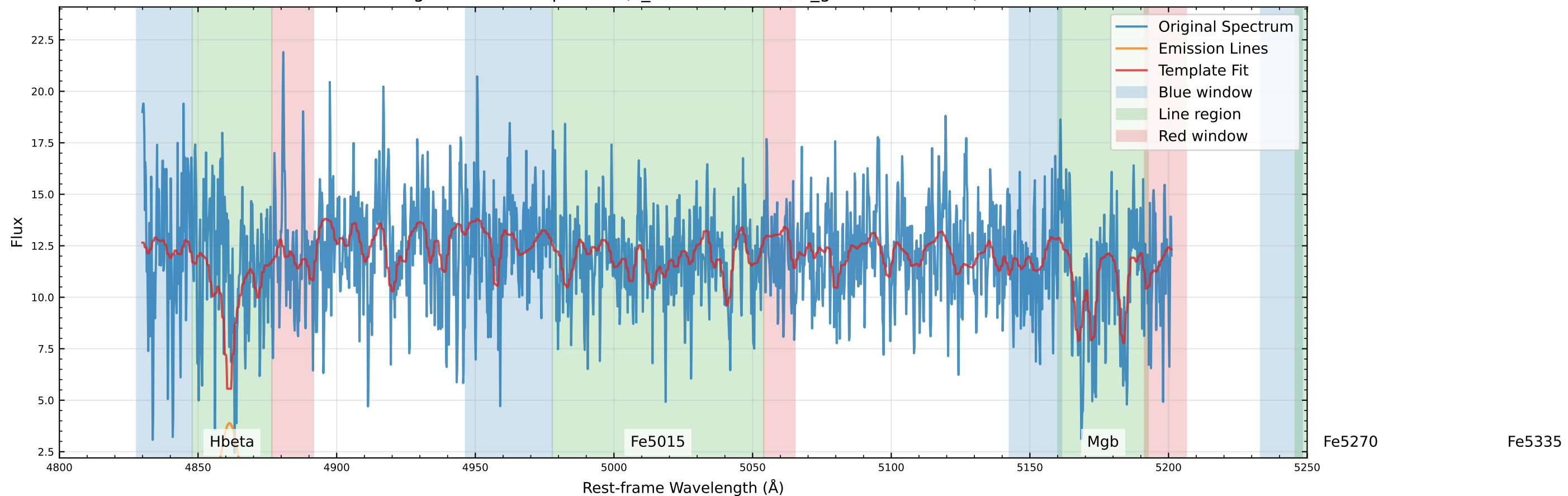
Original Data Comparison (v_star=41.3 km/s, v_gas=-118.6 km/s)
