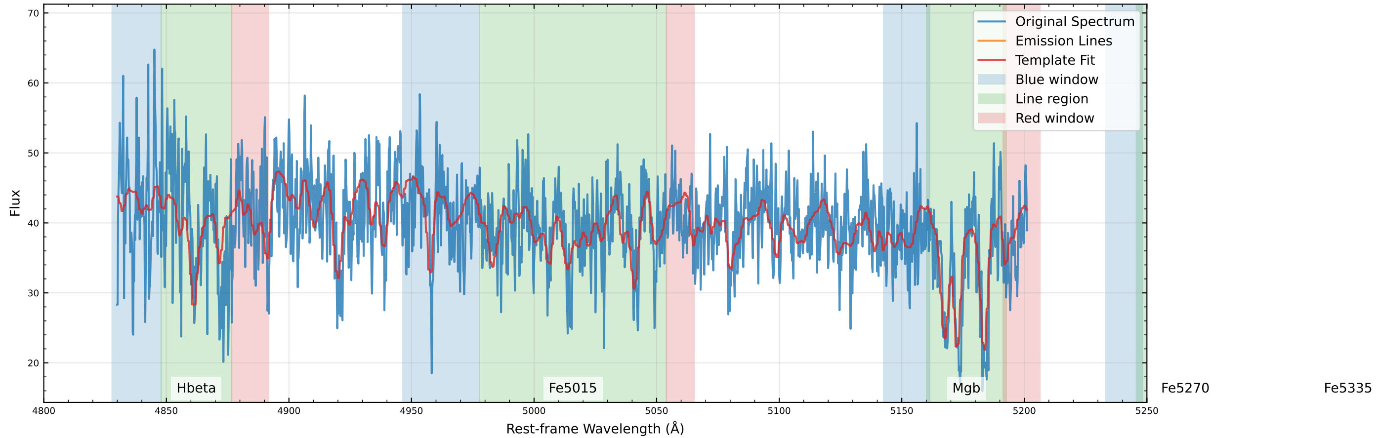
Original Data Comparison (v_star=28.1 km/s, v_gas=72.9 km/s)
