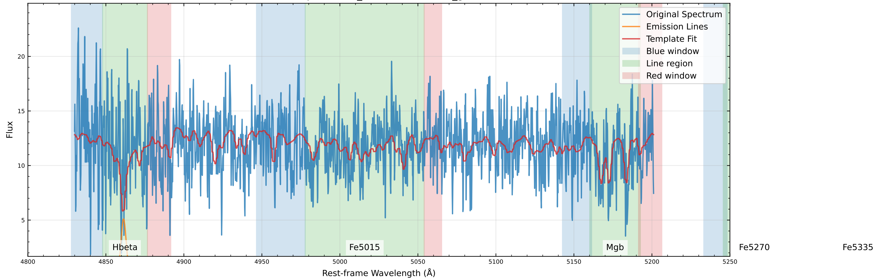
Original Data Comparison ( v_{\text{star}}=24.7 km/s, v_{\text{gas}}=126.2 km/s)
