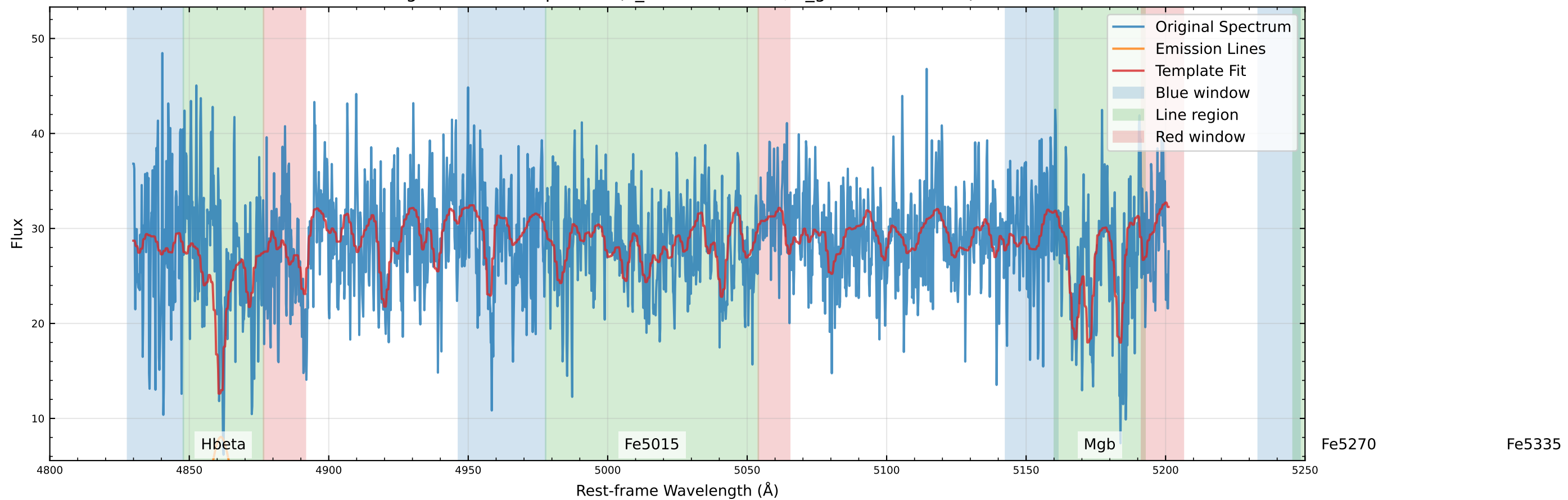
Original Data Comparison ( v_{\text{star}}=43.2 km/s, v_{\text{gas}}=-146.2 km/s)
