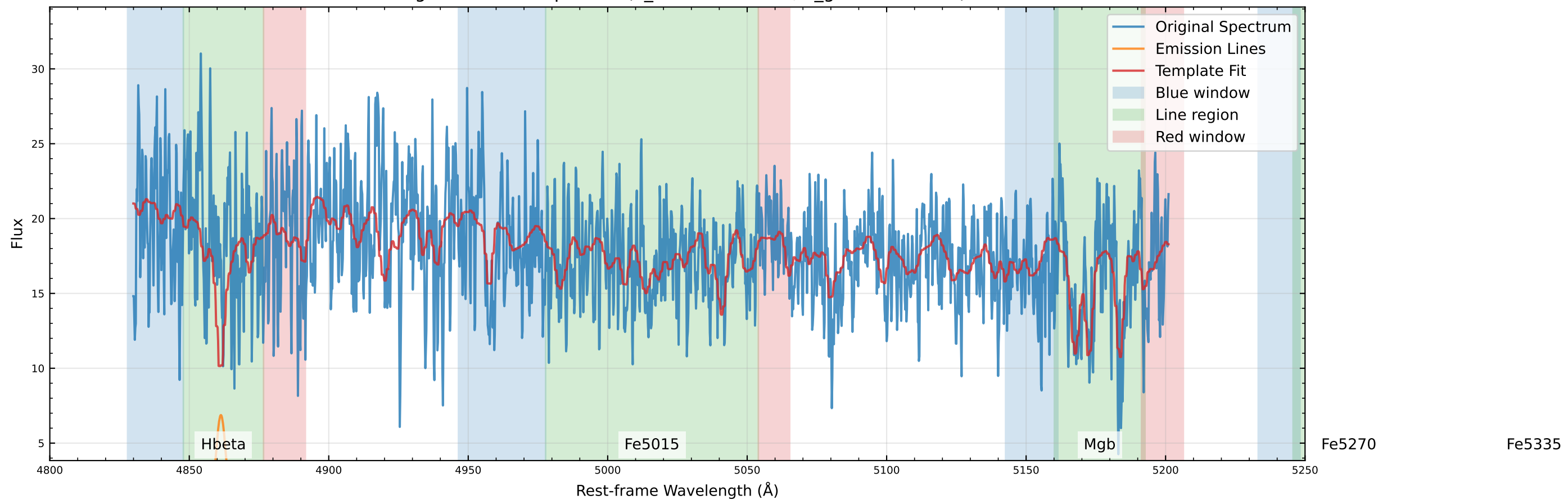
Original Data Comparison (v_star=46.4 km/s, v_gas=67.5 km/s)
