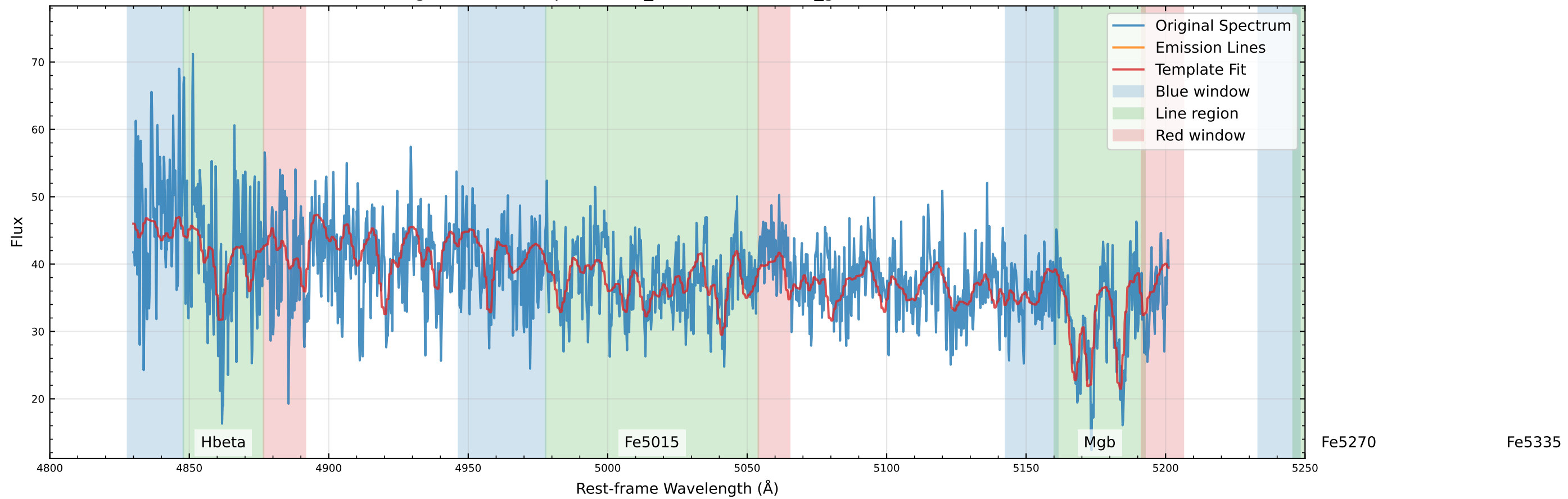
Original Data Comparison (v_star=51.1 km/s, v_gas=90.4 km/s)
