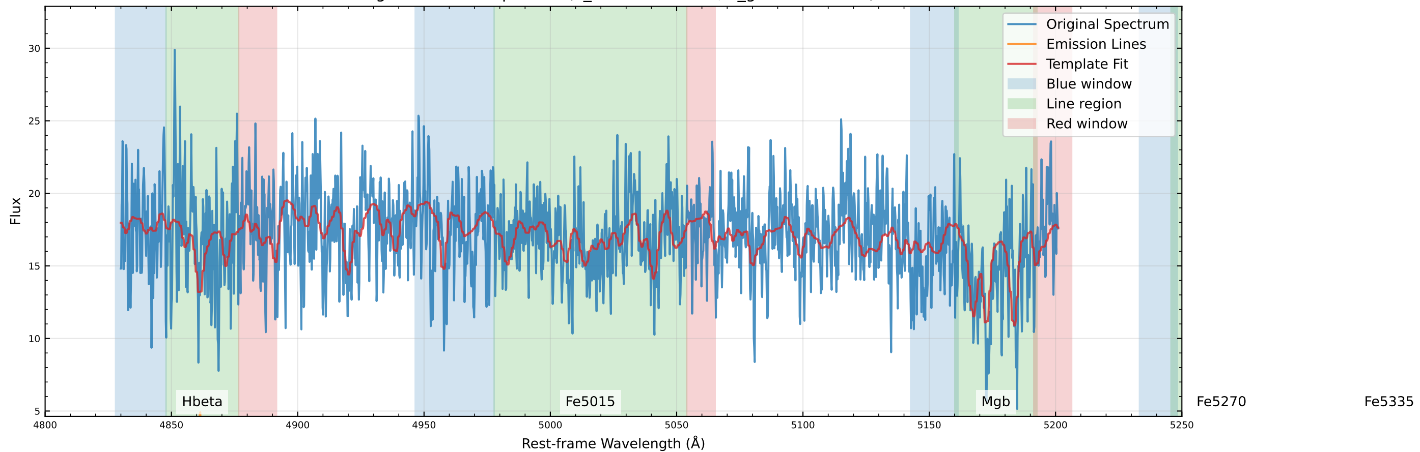
Original Data Comparison (v_star=38.3 km/s, v_gas=58.3 km/s)
