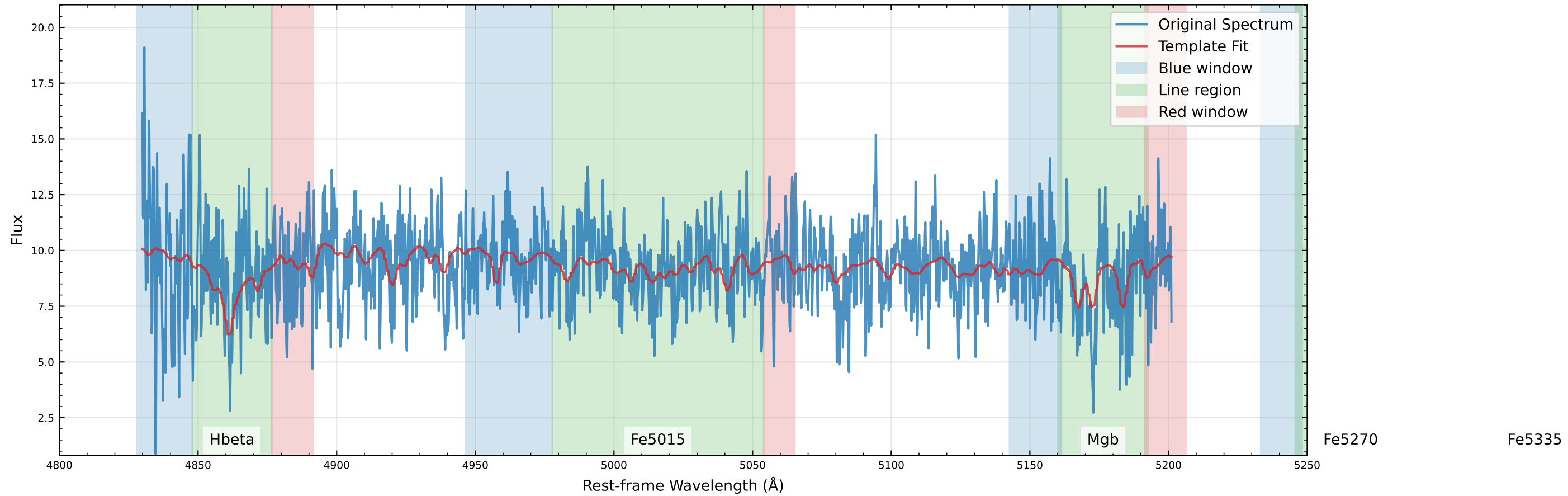
Original Data Comparison (v_star=37.8 km/s)
