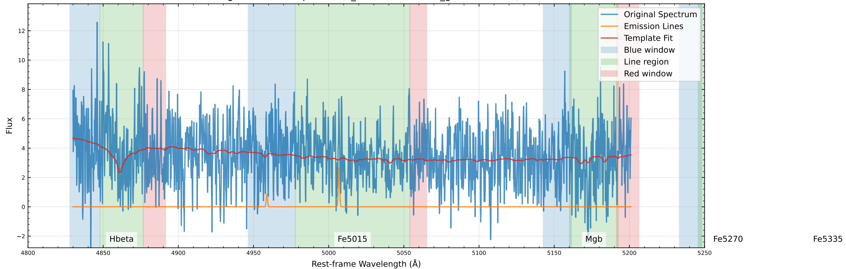
Original Data Comparison (v_star=-1.1 km/s, v_gas=-5.6 km/s)
