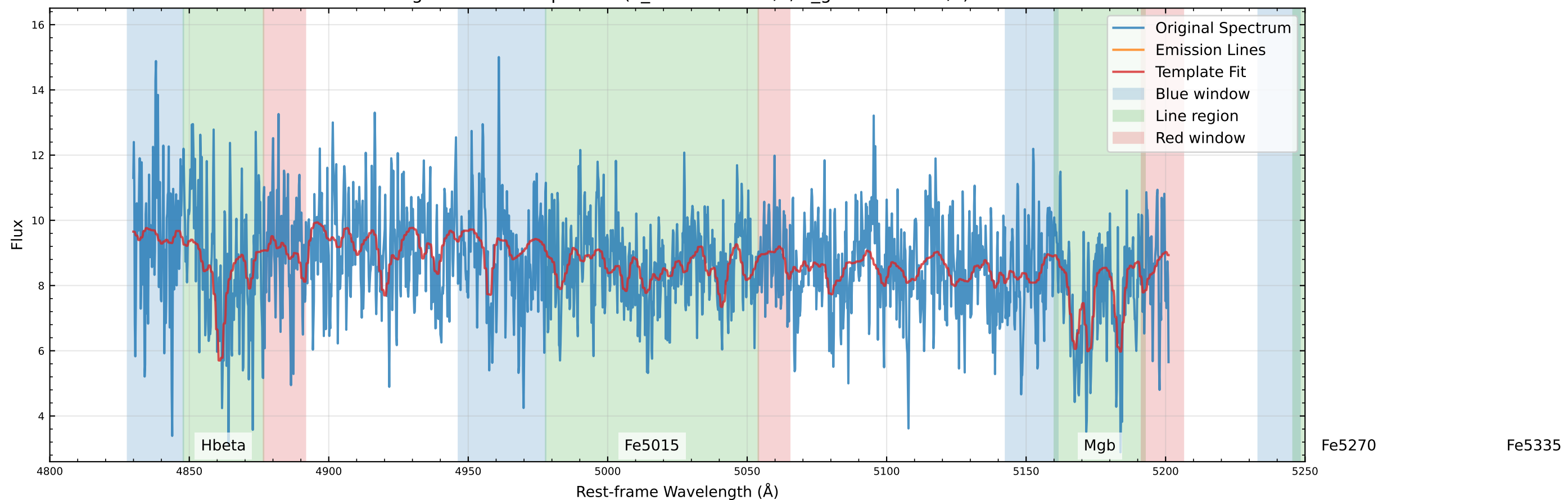
Original Data Comparison (v_star=26.7 km/s, v_gas=-10.7 km/s)
