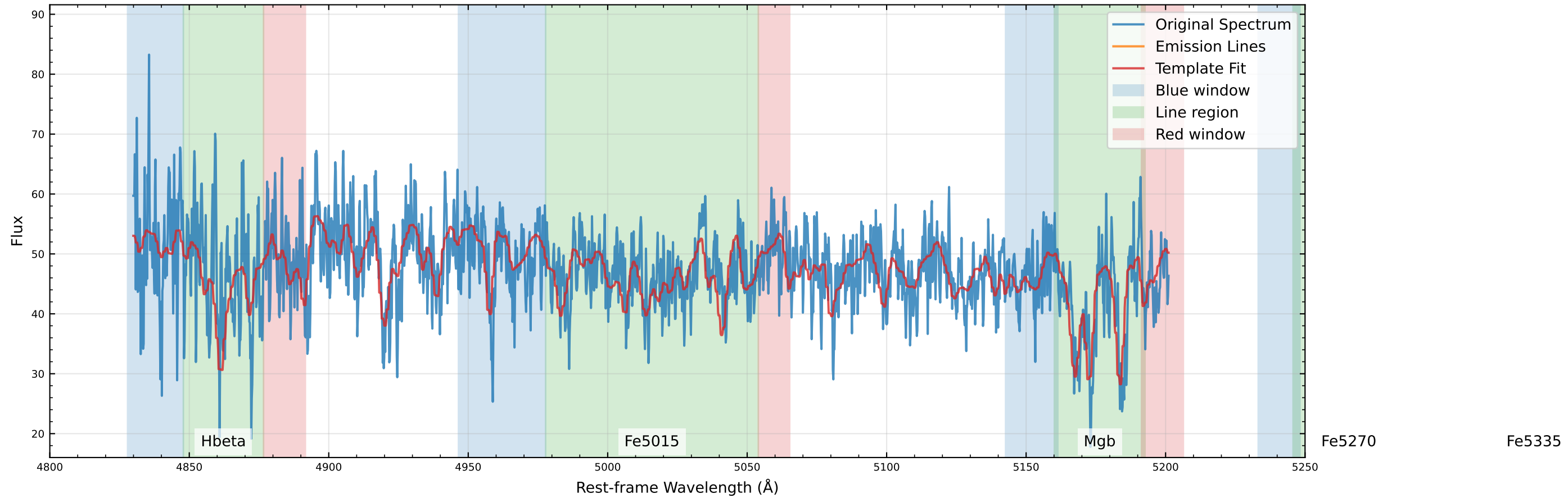
Original Data Comparison (v_star=48.5 km/s, v_gas=-2.5 km/s)
