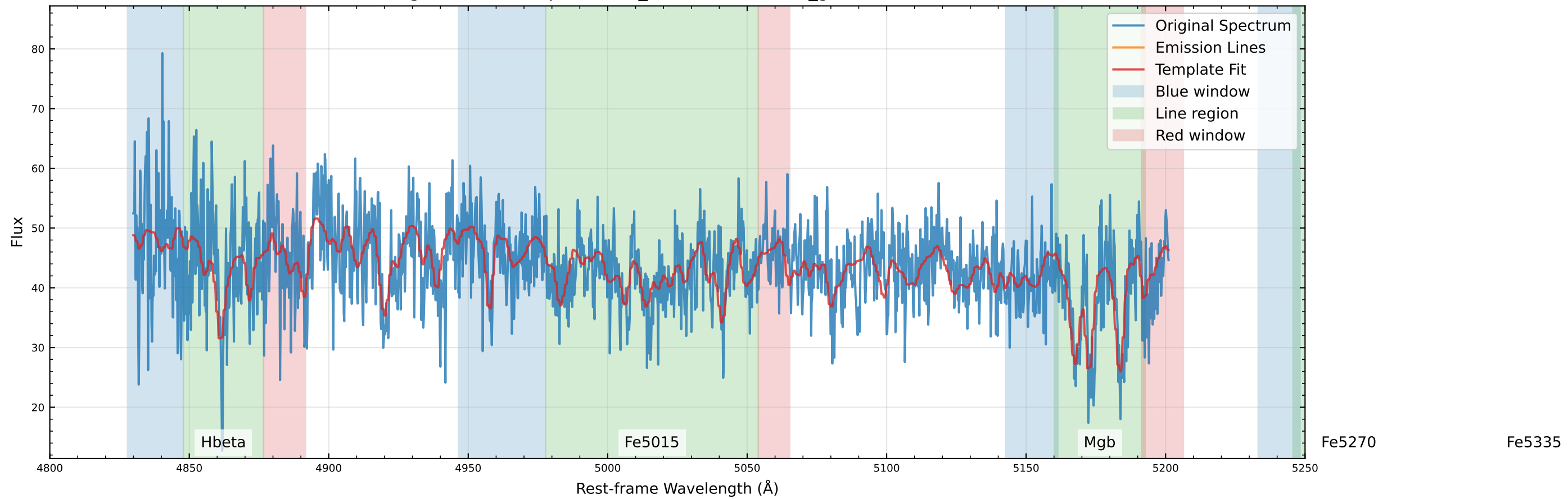
Original Data Comparison (v_star=44.1 km/s, v_gas=113.1 km/s)
