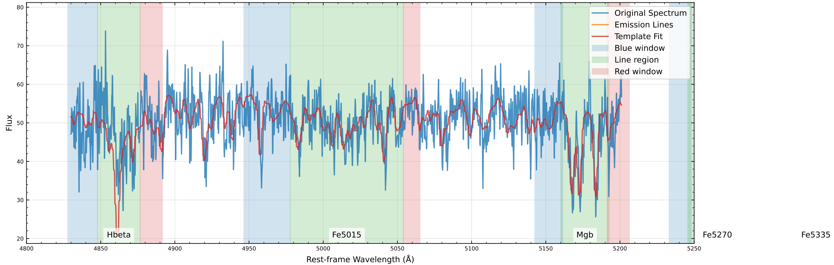
Original Data Comparison (v_star=32.6 km/s, v_gas=-46.0 km/s)
