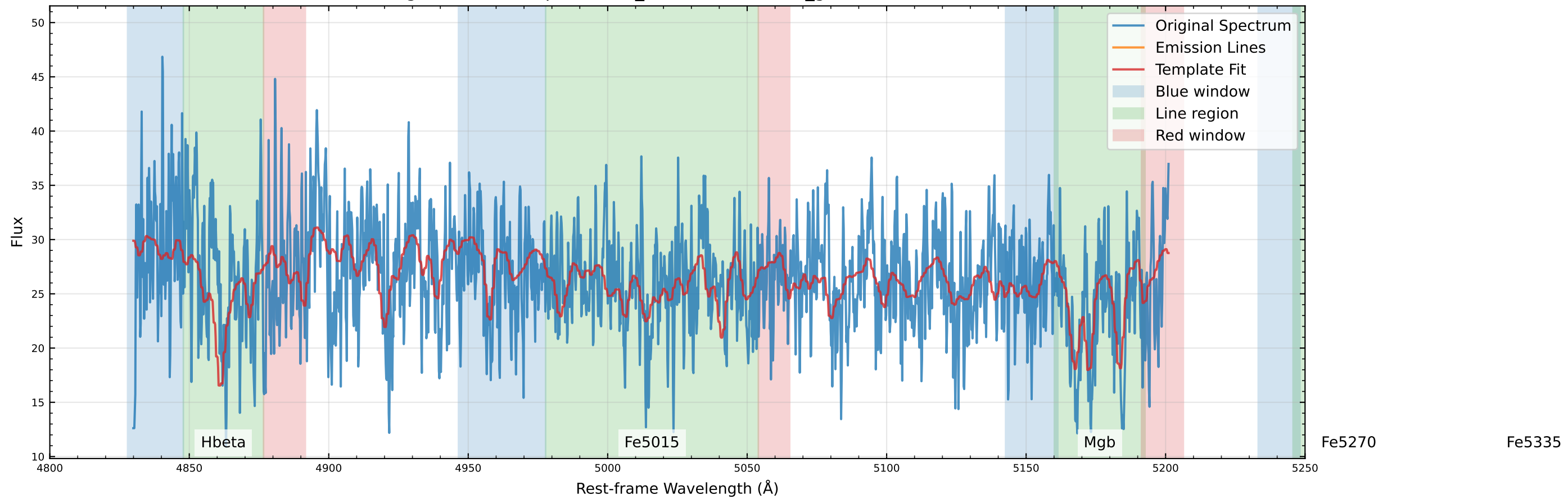
Original Data Comparison (v_star=49.1 km/s, v_gas=-122.0 km/s)
