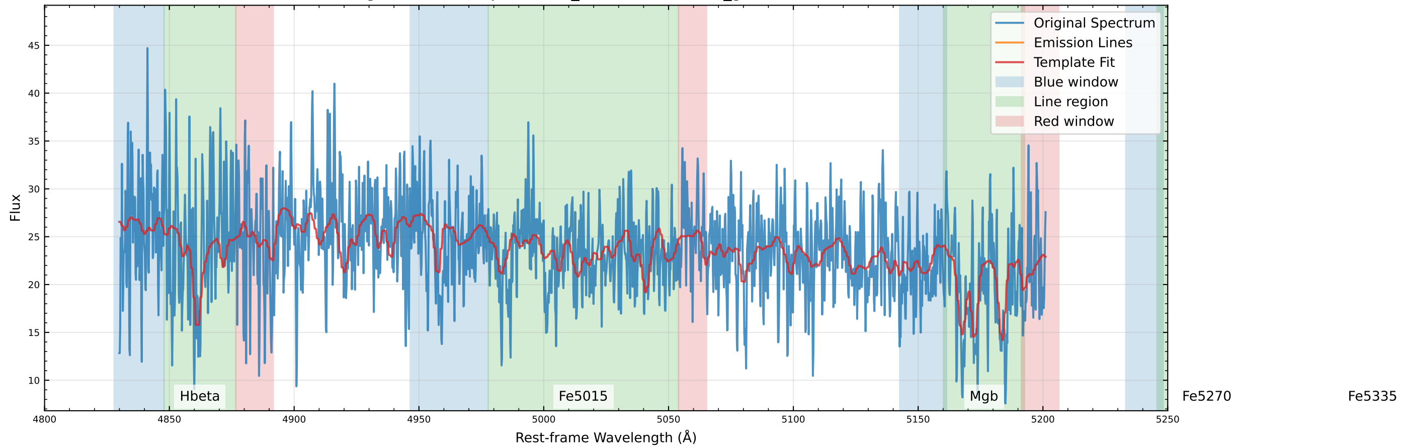
Original Data Comparison (v_star=32.6 km/s, v_gas=332.6 km/s)
