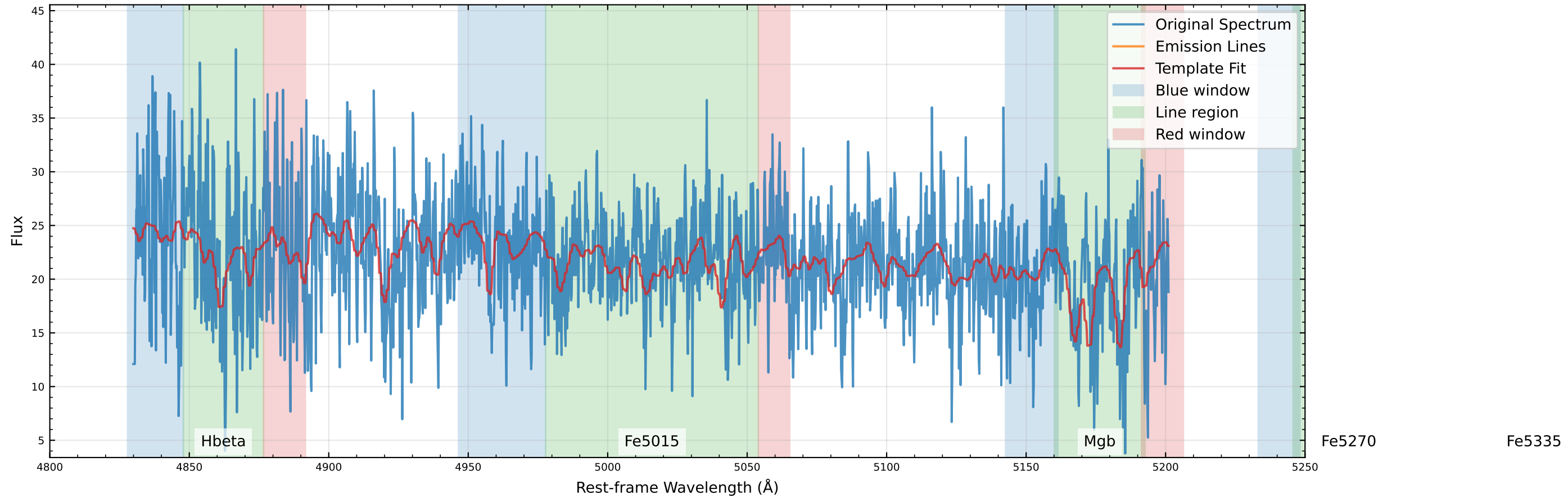
Original Data Comparison (v_star=65.4 km/s, v_gas=111.7 km/s)
