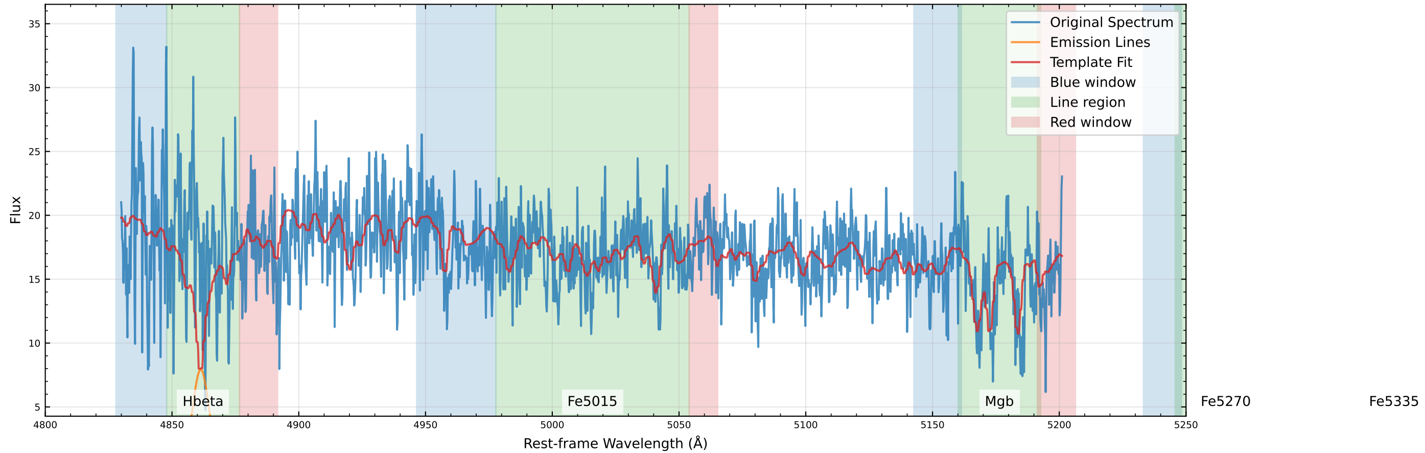
Original Data Comparison (v_star=59.2 km/s, v_gas=-73.1 km/s)
