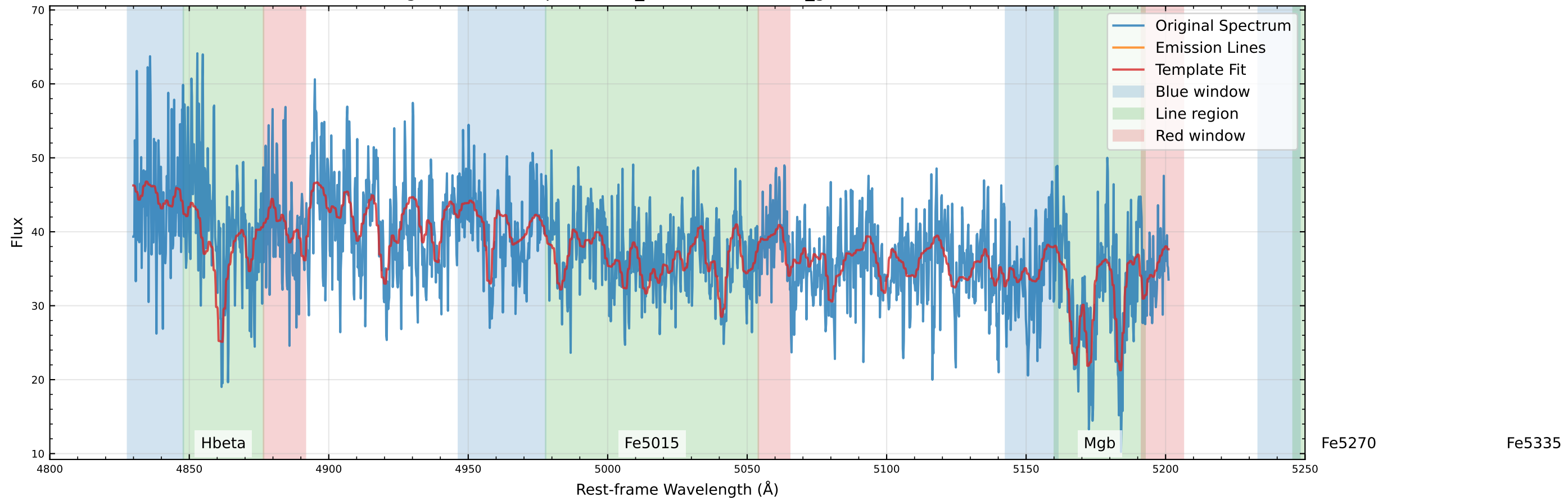
Original Data Comparison (v_star=42.8 km/s, v_gas=-256.1 km/s)
