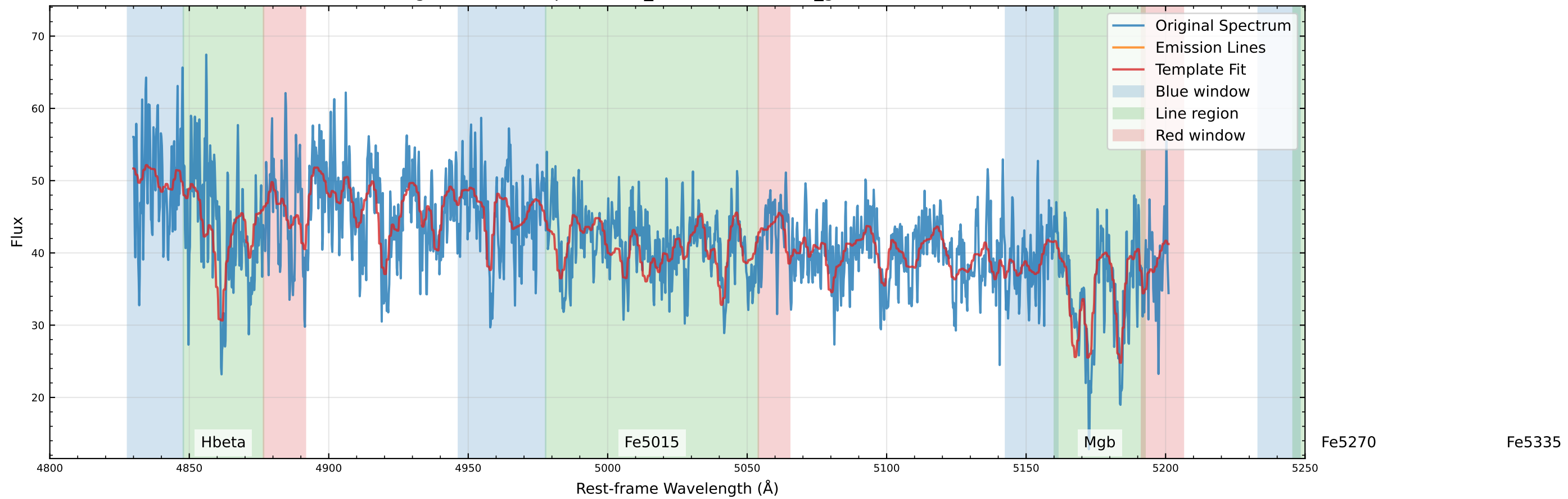
Original Data Comparison (v_star=33.6 km/s, v_gas=80.1 km/s)
